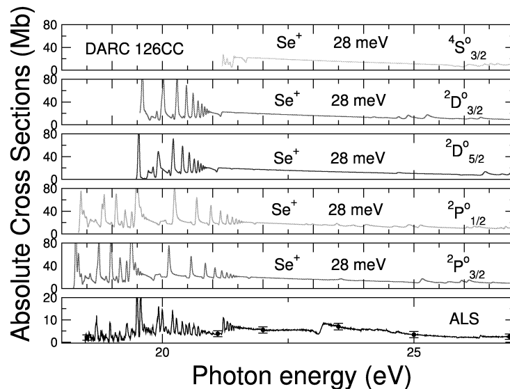
Figure 6: Theoretical Se + PI cross-sections (upper panels) computed from 126-level close-coupling DARC calculations (Sterling et al. 2009), convoluted with a Gaussian to the experimental FWHM resolution of 28 meV. The cross-section of each state in the ground configuration is shown, and compared to the experimental cross-section (bottom panel).
