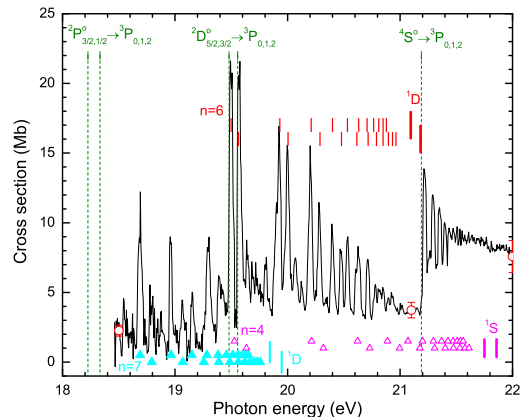
Figure 4: Top panel: The \text{Se}^+ photoionization cross-section measured at the ALS (Sterling et al. 2009). The circles with error bars represent absolute measurements performed at discrete photon energies. Bottom panel: Magnified view of the \text{Se}^+ PI cross-section in the metastable region (the ground state ionization threshold is at 21.2 eV), with resonances and Rydberg series identified.
